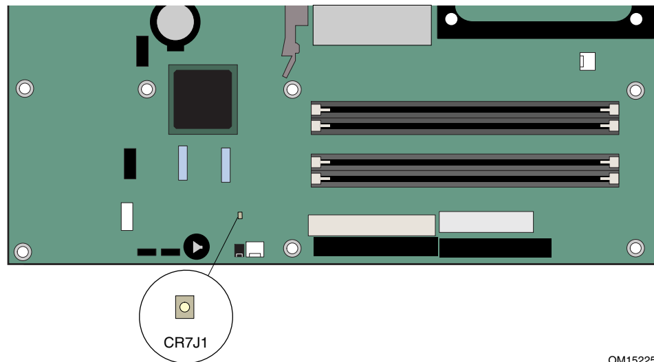
Figure 2. Location of Standby Power Indicator
